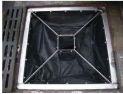
DROP INLET WITH CENTER PORT
